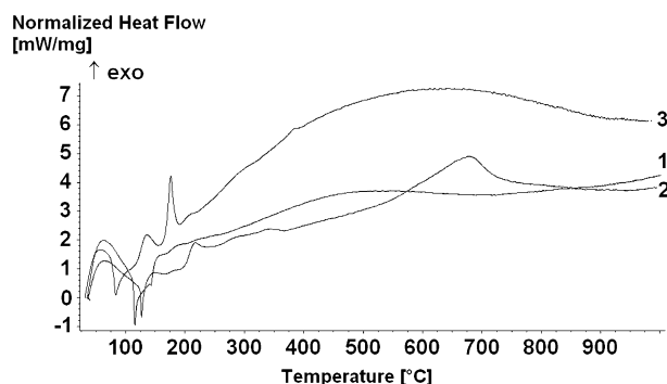
Fig. 2 DSC plots of compounds 1–3.
