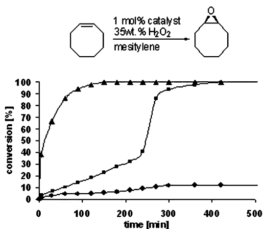
Fig. 8 Time-conversion diagram of the epoxidation of cis -cyclooctene with 1 (▲), 2 (■) and 3 (●) as catalyst precursor.
