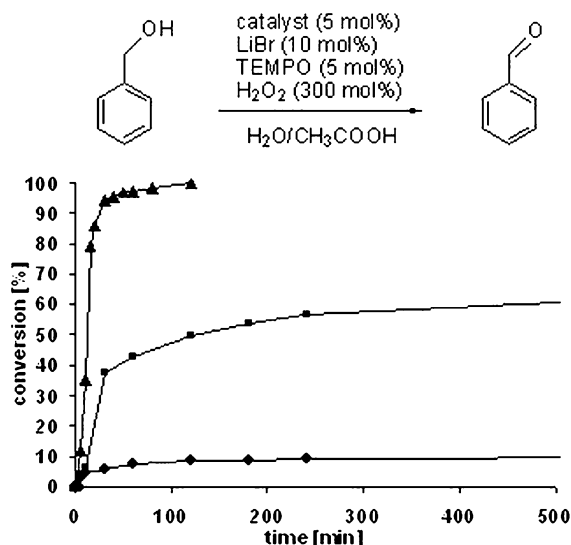
Fig. 9 Time-conversion diagram of the oxidation of benzyl alcohol with 1 (▲), 2 (■) and 3 (●) as catalyst precursor.
