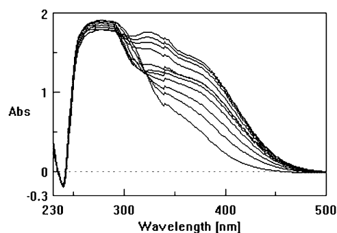
Fig. 7 UV-vis spectra of compound 3 , treated with hydrogen peroxide (see text).
