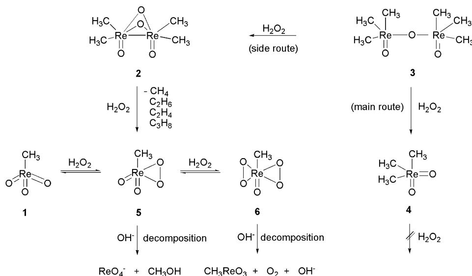
Scheme 2 Reaction of compounds 1–3 with \text{H}_2\text{O}_2 .
