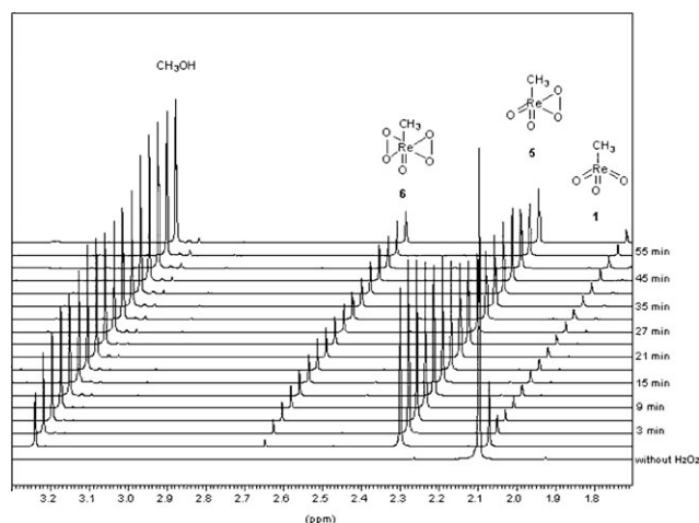
Fig. 3 ^1\text{H} NMR kinetic study of the reaction of compound 1 with \text{H}_2\text{O}_2 .
