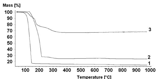
Fig. 1 TG spectra of compounds 1–3.
