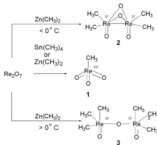
Scheme 1 Reaction of \text{Re}_2\text{O}_7 with dimethylzinc.
