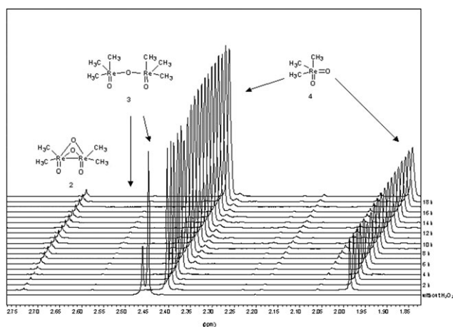
Fig. 5 ^1\text{H} NMR kinetic study of the reaction of compound 3 with \text{H}_2\text{O}_2 .
