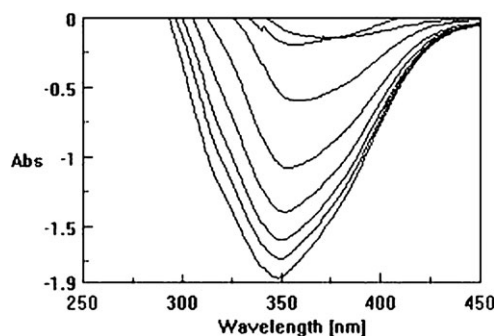
Fig. 6 The formation of compound 6 from the reaction of 2 with \text{H}_2\text{O}_2 (difference spectrum to emphasize the changes); see text for more details.
