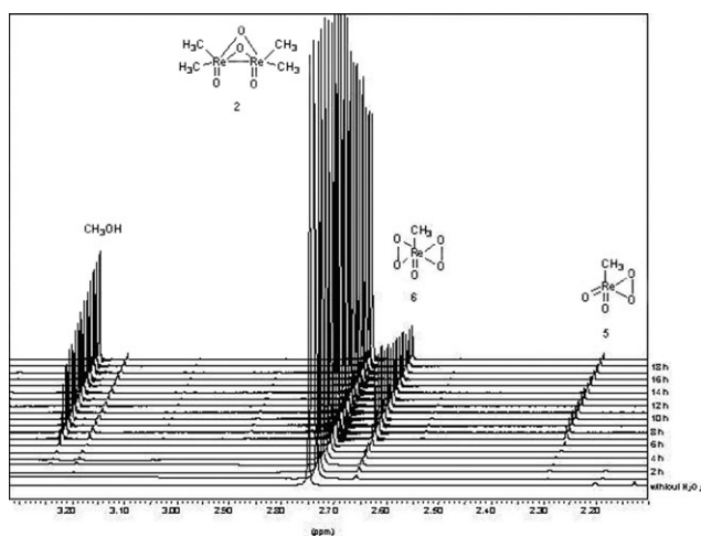
Fig. 4 ^1\text{H} NMR kinetic study of the reaction of compound 2 with \text{H}_2\text{O}_2 .
